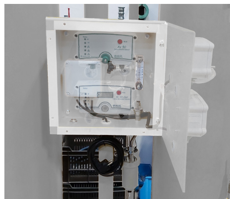
BM sensing panel (includes O 2 , CO, CO 2 monitoring)
